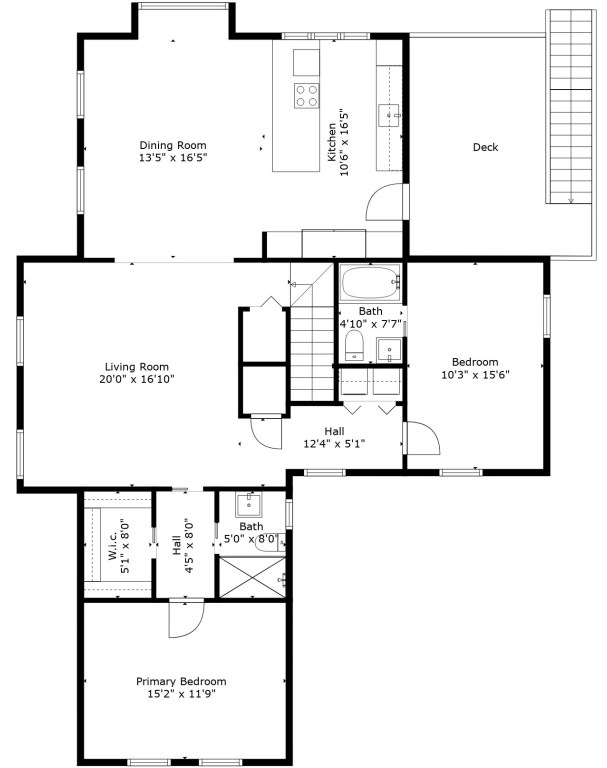
Upper Level
